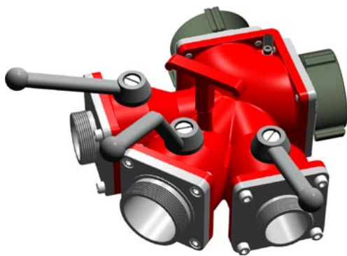
TRIPOK VALVE WITH TWO INLETS
