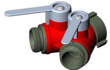
BIPOK WILDLAND 1.5" NST / 2x1.5" NST long handle *Available Long or Short Handle
